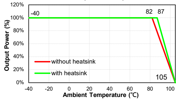
EC2SBW-XXD15H Derating Curve (Vin=Nominal)
